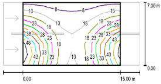
Luminance Distribution
