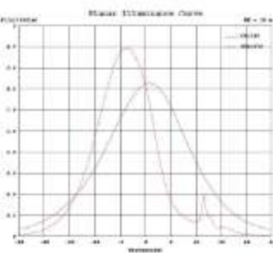
Illumination Curve
